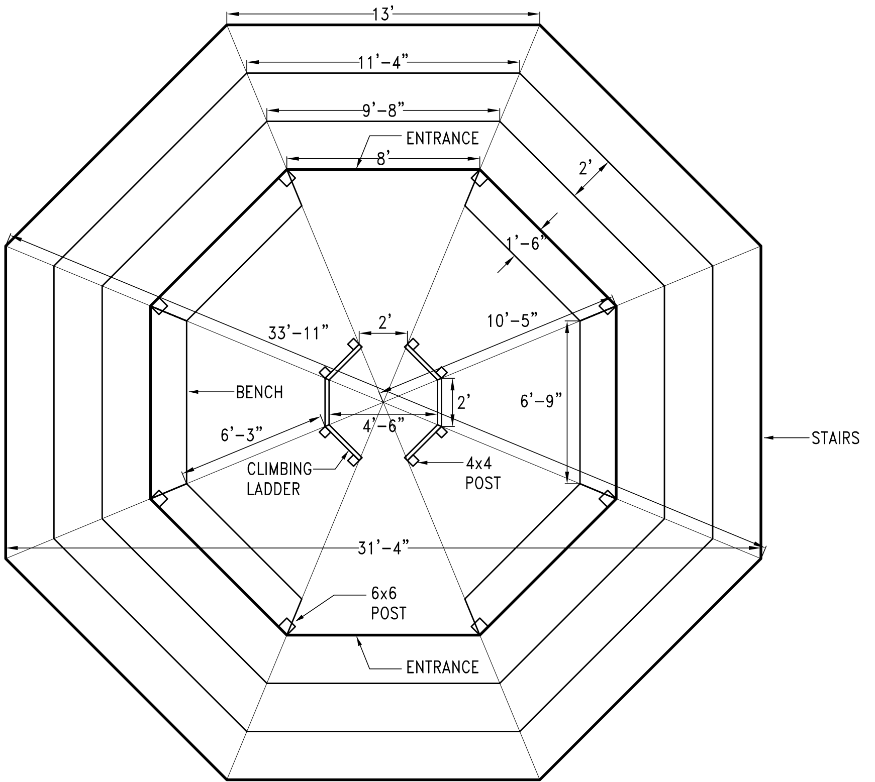
2 GROUND FLOOR PLAN - FLOOR LEVEL 1/4" = 1'-0"
